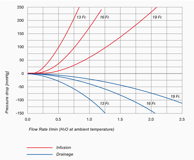
Pressure drop vs. flow 13, 16, 19 Fr.
