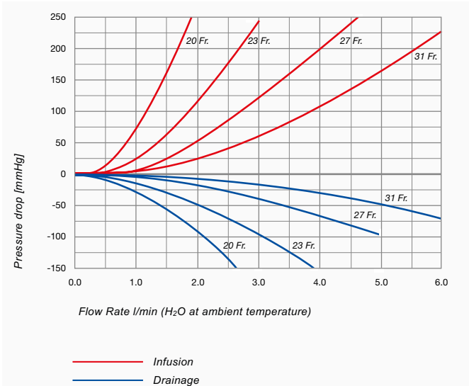
Pressure drop vs. flow 20, 23, 27, 31 Fr.
